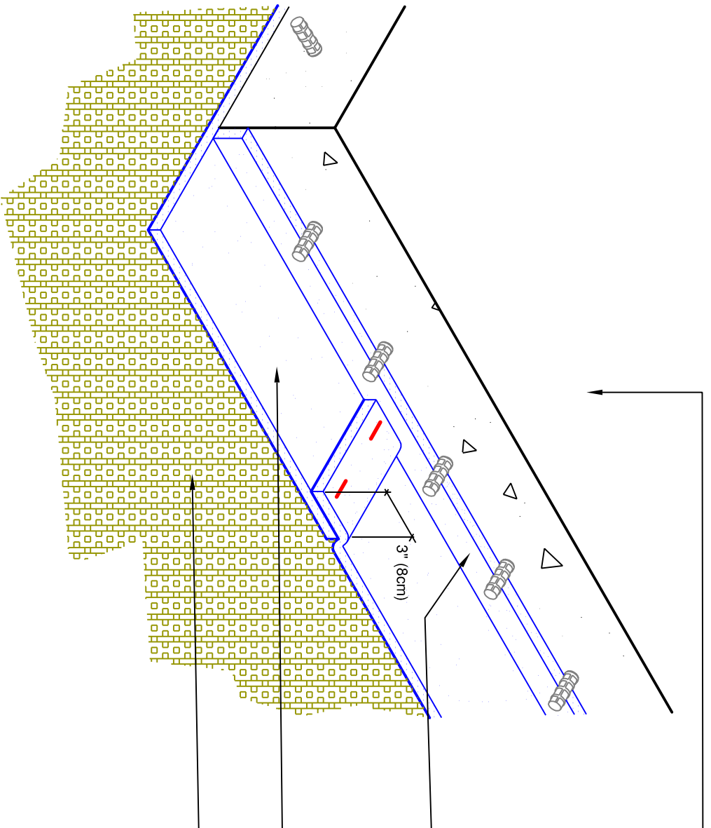
Simple Slab - System A (Also See BSOG-01).
