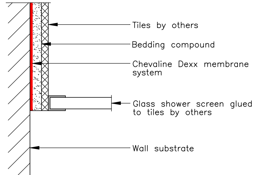
Shower Screen/Wall Junction
