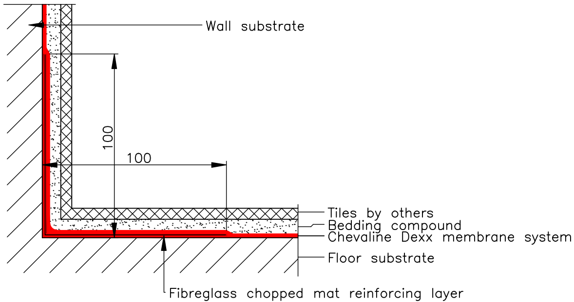
Wall/Floor Junction
